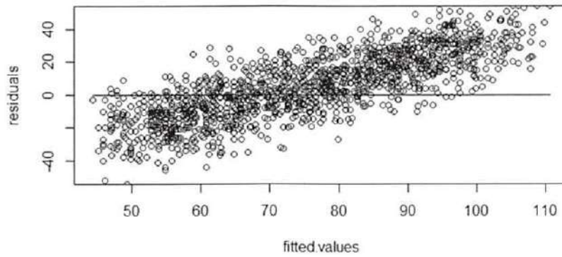
FIGURE 6-9 Residuals with a linear trend
