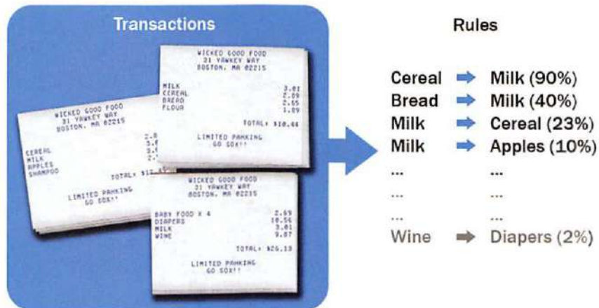
FIGURE 5-1 The general logic behind association rules
