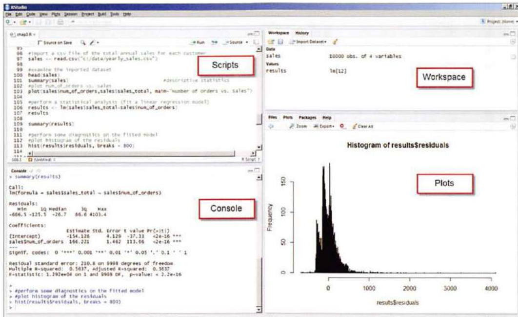
FIGURE 3-3 RStudio GUI
